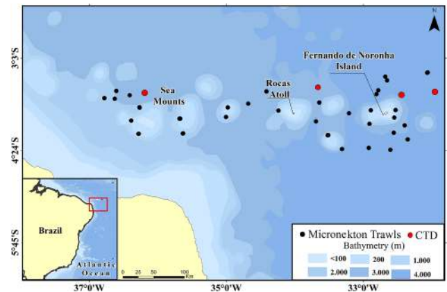
Fig. 1. Study area with the CTD and micronekton-trawl sampling stations.
