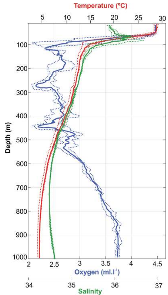
Fig. 2. Mean and standard deviation of vertical profiles of temperature (red), salinity (green) and dissolved oxygen (blue) off oceanic islands of the western Tropical Atlantic between April and May 2017.
