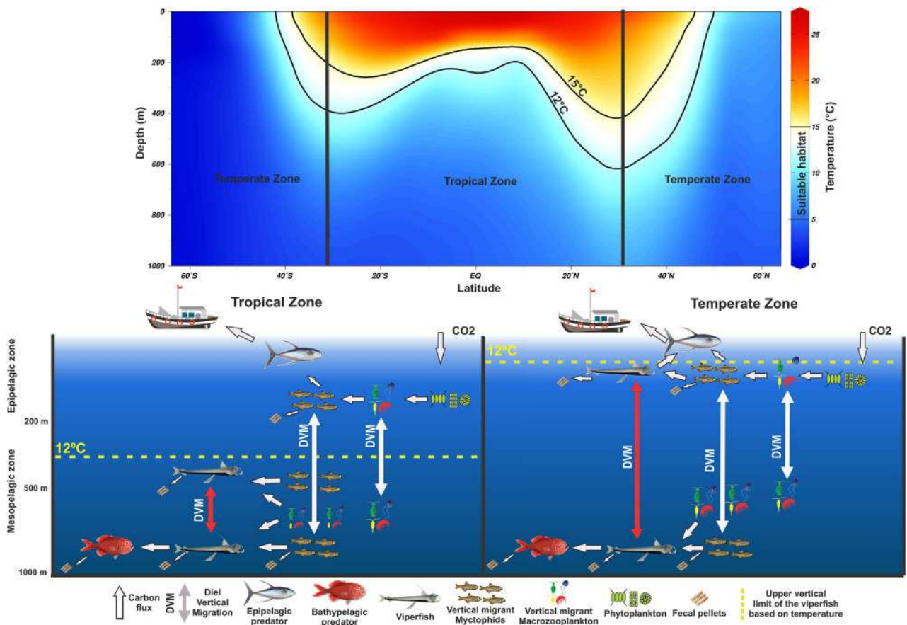
Figure 7. Conceptual model exhibiting global suitable vertical habitat of the viperfish Chauliodus sloani based on temperature profiles (Source: Word Ocean Atlas 73 ) and differences in the vertical migration and trophic interactions of this species in the tropical and temperate waters. Temperature information from the upper panel refers to the meridional Sect. 30°.
