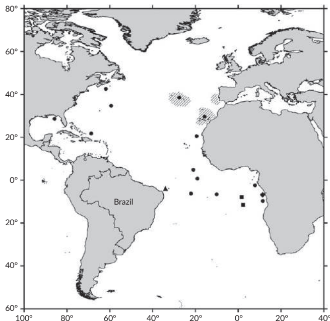
FIGURE 2 Distribution of Aphanopus intermedius based on literature, Biscoito et al. (2011; ■), Parin (1994; ●), Vasil'eva et al. (2001; ◆), Pakhorukov et al. (2014; ■) and the present study (▲)
