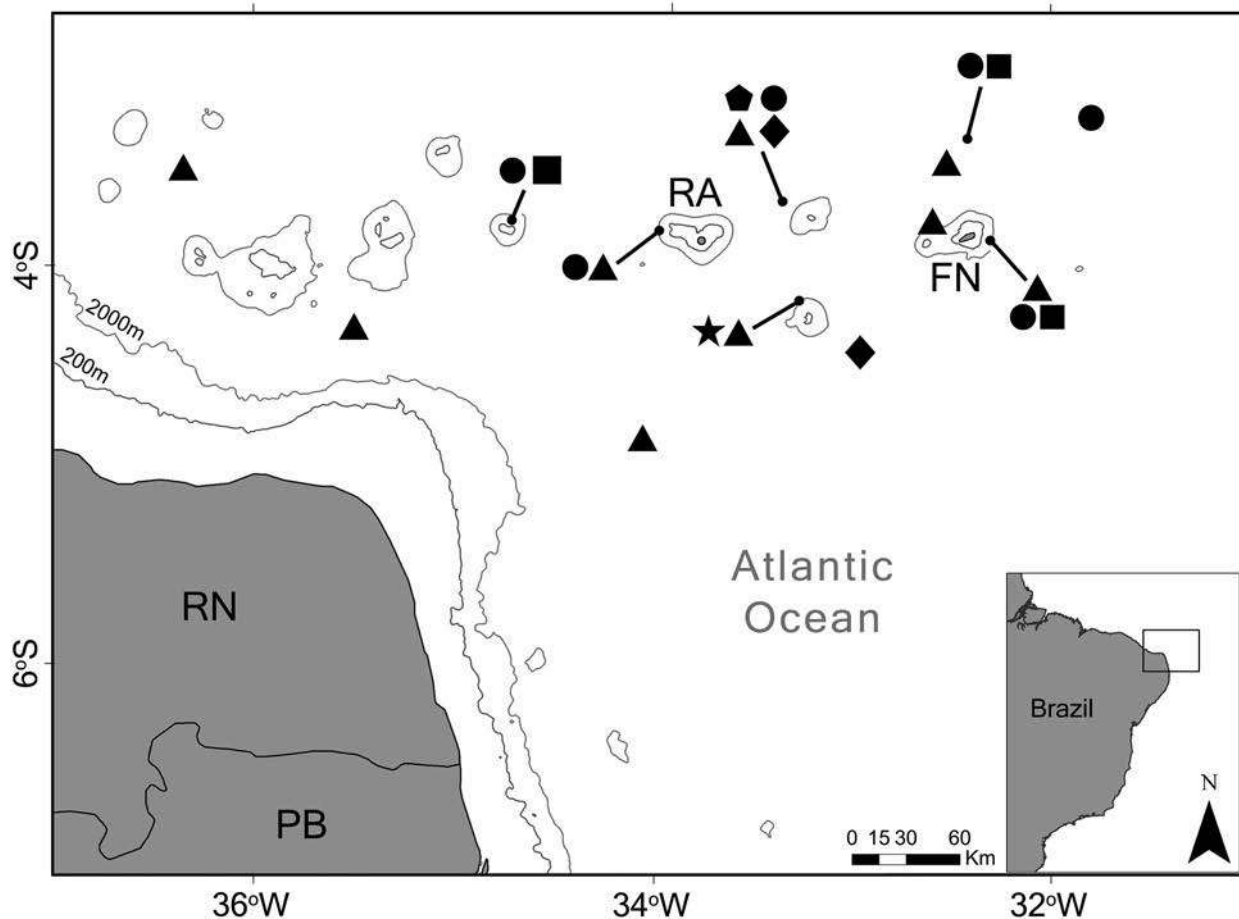
Figure 2. Records of Argentiniformes off northeastern Brazil based on specimens collected during the ABRACOS 2 expedition: Dolicholagus longirostris (circle), Melanolagus bericoides (square), Xenophthalmichthys danae (diamond), Opisthoproctus soleatus (pentagon), Rhynchohyalus natalensis (star), Winteria telescopa (triangle). The small circle at the end of the lines indicates the same trawl haul for different species. FN – Fernando de Noronha Archipelago; PB – Paraíba; RA – Rocas Atoll; RN – Rio Grande do Norte.
