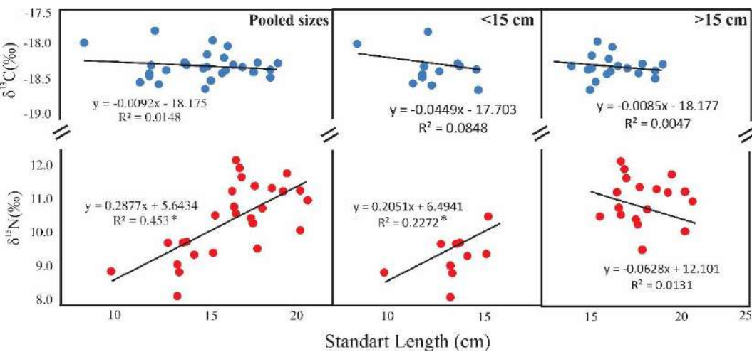
Supplementary Material 2 – Results of least-squares regression analysis between standard length (cm) and \delta^{15}\text{N} and \delta^{13}\text{C} values of the viperfish Chauliodus sloani . * relationships presenting significant statistical differences ( p < 0.05 ).
