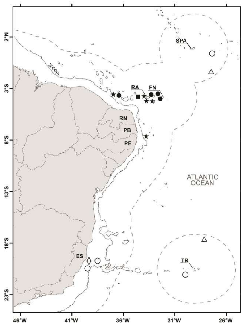
FIGURE 3 | Records of the Melanocetidae and Thaumichthyidae in Brazilian waters: Melanocetus johnsonii (circle), Melanocetus murrayi (triangle), Melanocetus sp. (star), Thaumichthys binghami (diamond), Thaumichthys sp. (square). Full symbols represent specimens collected during the ABRACOS surveys and open symbols are records from the literature (see text). Selected Brazilian States and islands are: Rio Grande do Norte, PB – Paraíba, PE – Pernambuco; ES – Espírito Santo; SPA – Saint Peter and Saint Paul Archipelago, FN – Fernando de Noronha Archipelago, RA – Rocas Atoll, TR – Trindade Island. Dashed line represents the outer limit of the Brazilian Exclusive Economic Zone.
